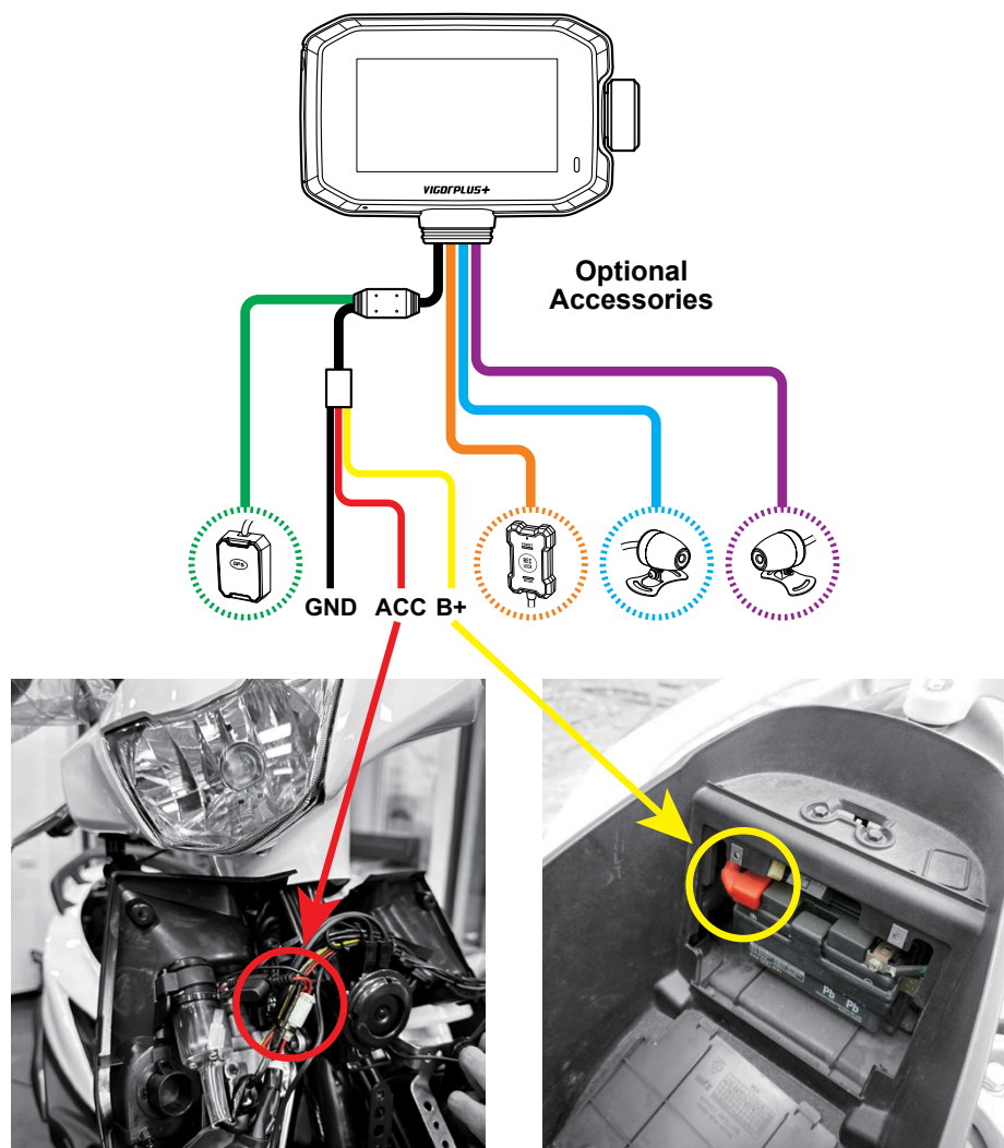
[Hardwire Kit Installation Diagram]
