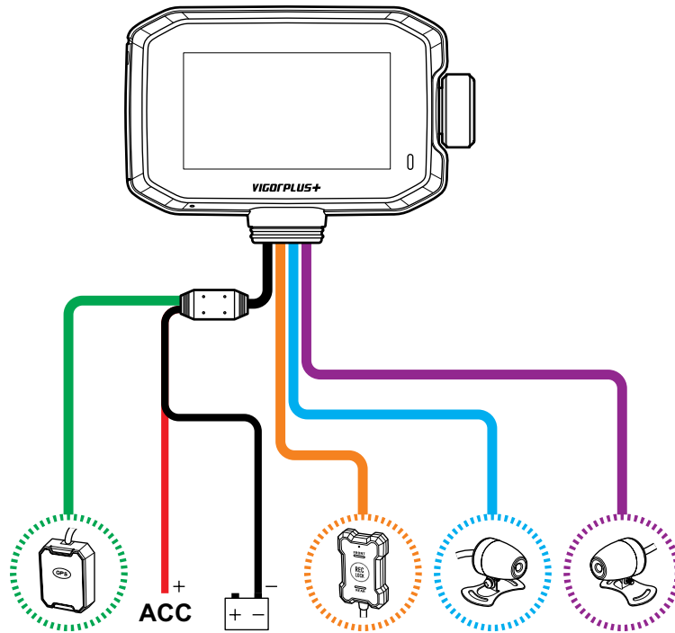
[Power Cable Installation Diagram]
