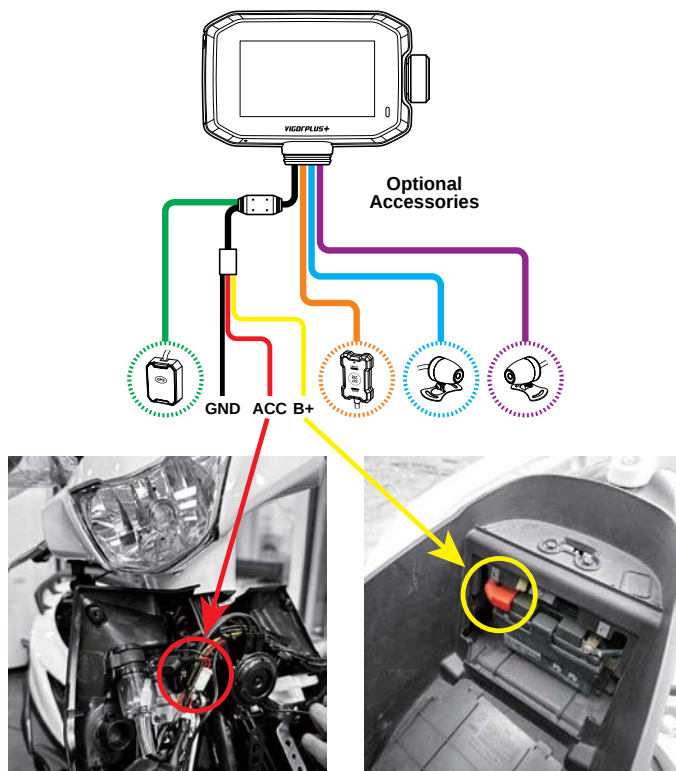
[Hardwire Kit Installation Diagram]
